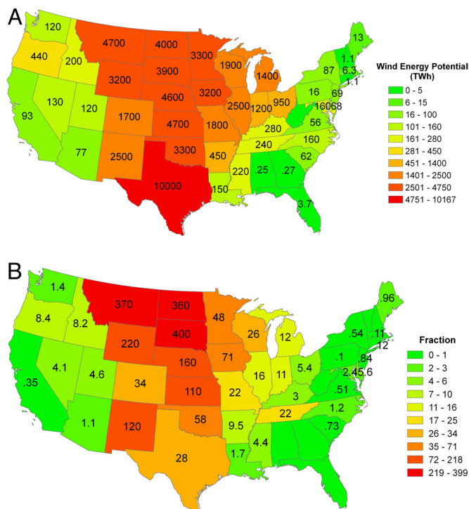
Fig. 5. Annual onshore wind energy potential on the state-by-state basis for the contiguous U.S. expressed in TWh (A) and as a ratio with respect to retail sales in the states (2006) (B). For example, the potential source for North Dakota exceeds current total electricity retail sales in that state by a factor of 360. Data source for total electricity retail sales was www.eia.doe.gov .
